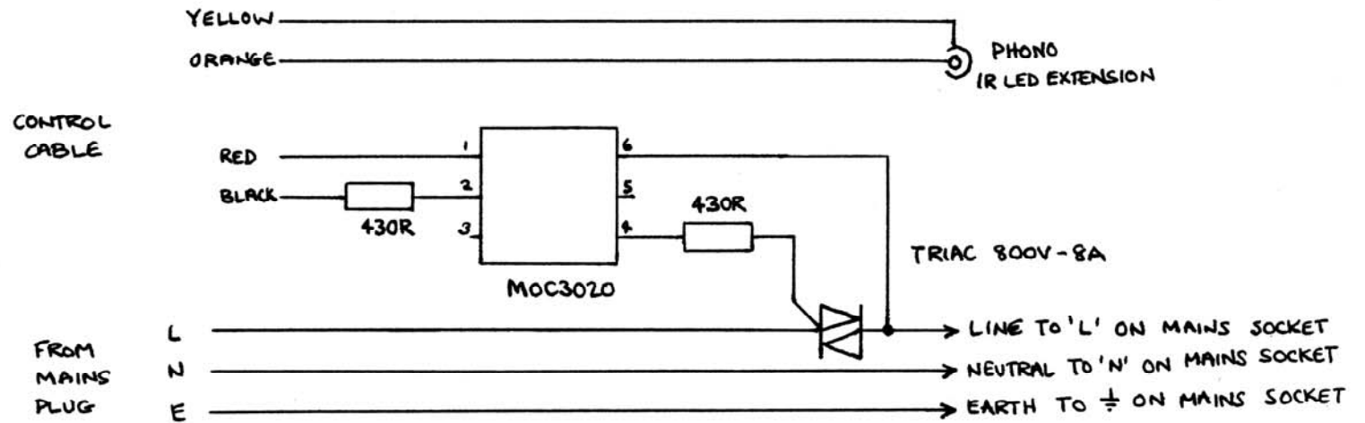
VCR POWER SWITCH
